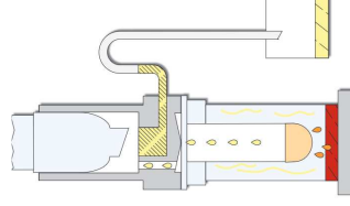
Stage 3: Extraction in solvent vapour with reflux
