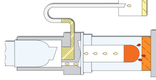
Stage 2: Solvent reduction, collection of distillate
