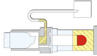
Stage 1: Extraction in boiling solvent
