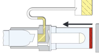
Stage 5: Lifting the cup, gentle evaporation
